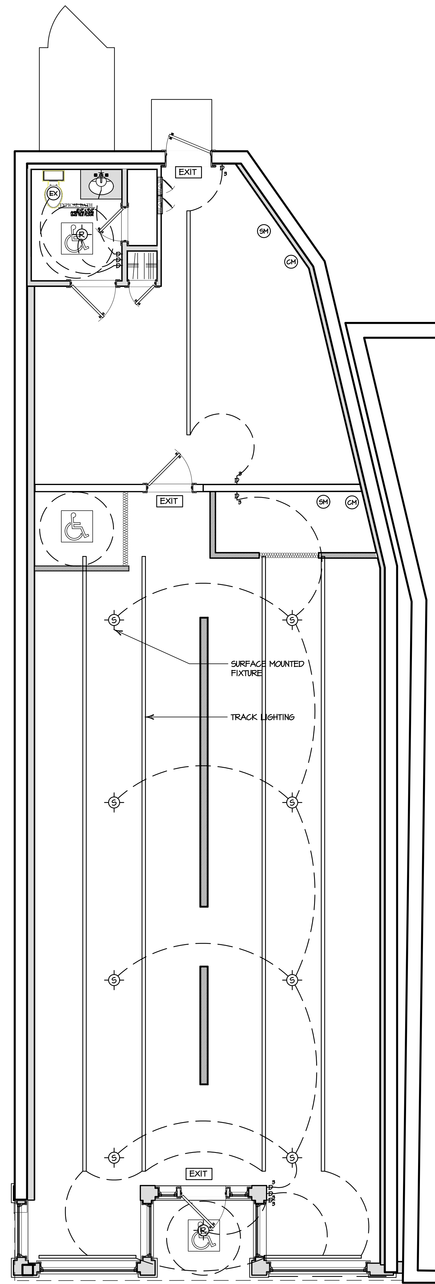
ELECTRICAL PLAN
