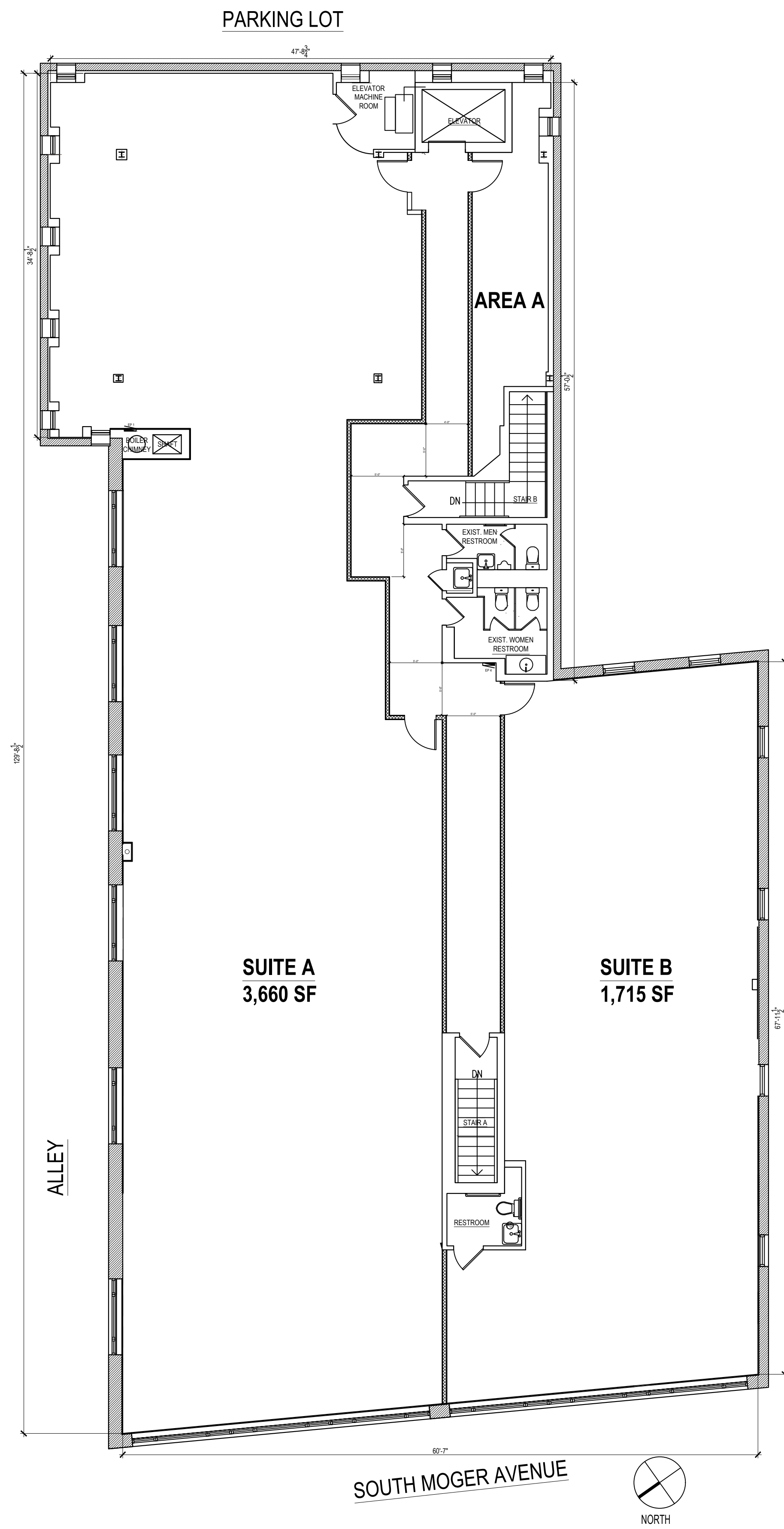
2ND FLOOR PLAN
